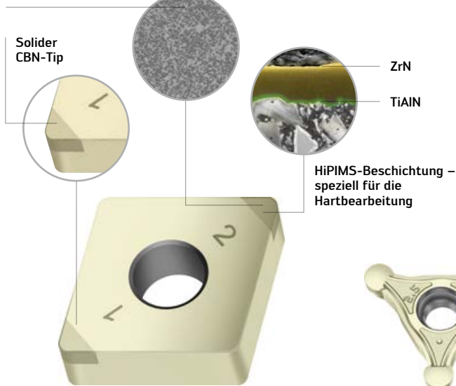
WBH20C ISO Wendeplatte Abb.: CNGA120408TM-2 WBH20C
